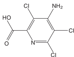
4-amino-3,5,6-trichloropicolinic acid
