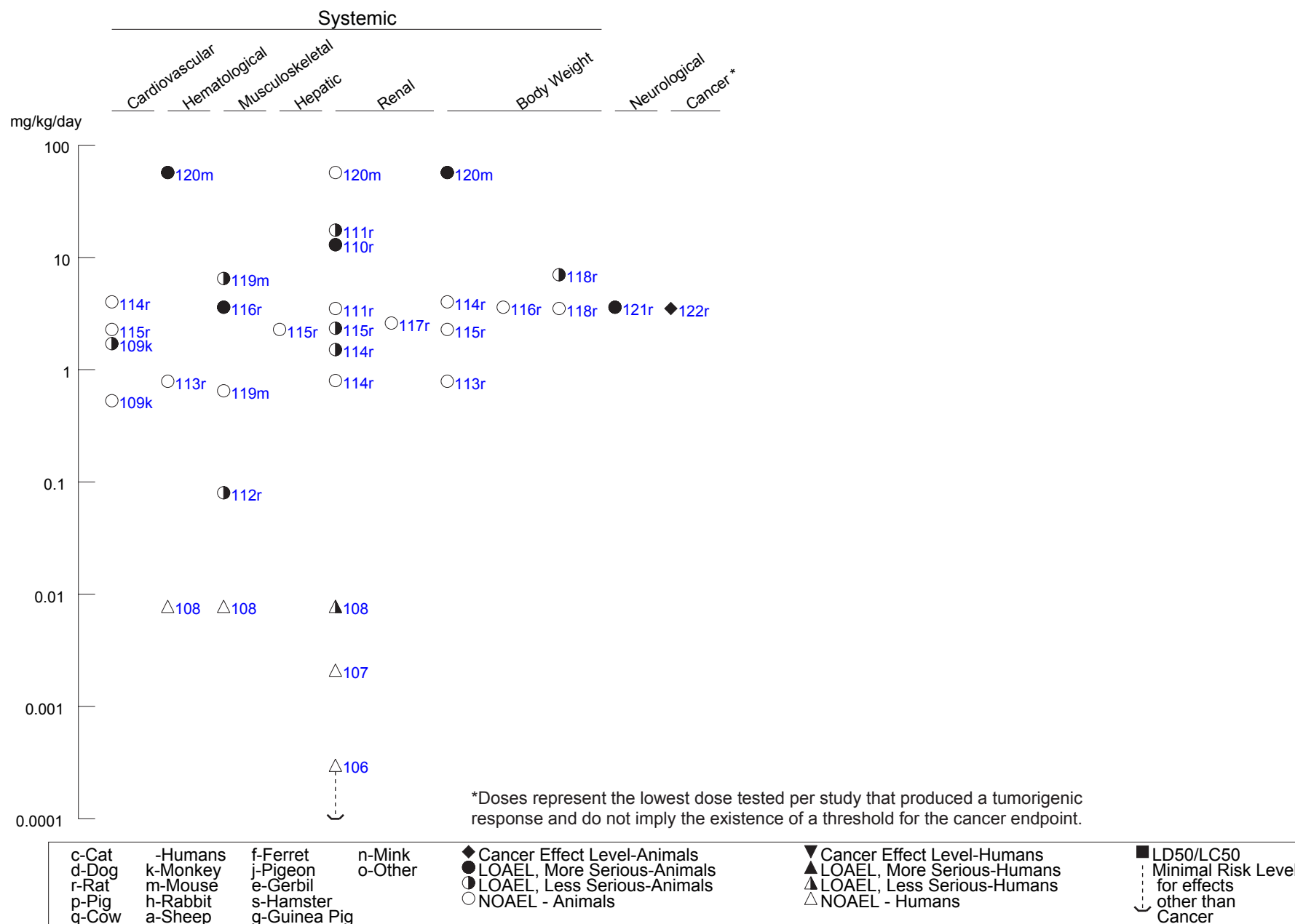
Figure 3-2 Levels of Significant Exposure to Cadmium - Oral ( Continued ) Chronic ( \geq 365 days)
