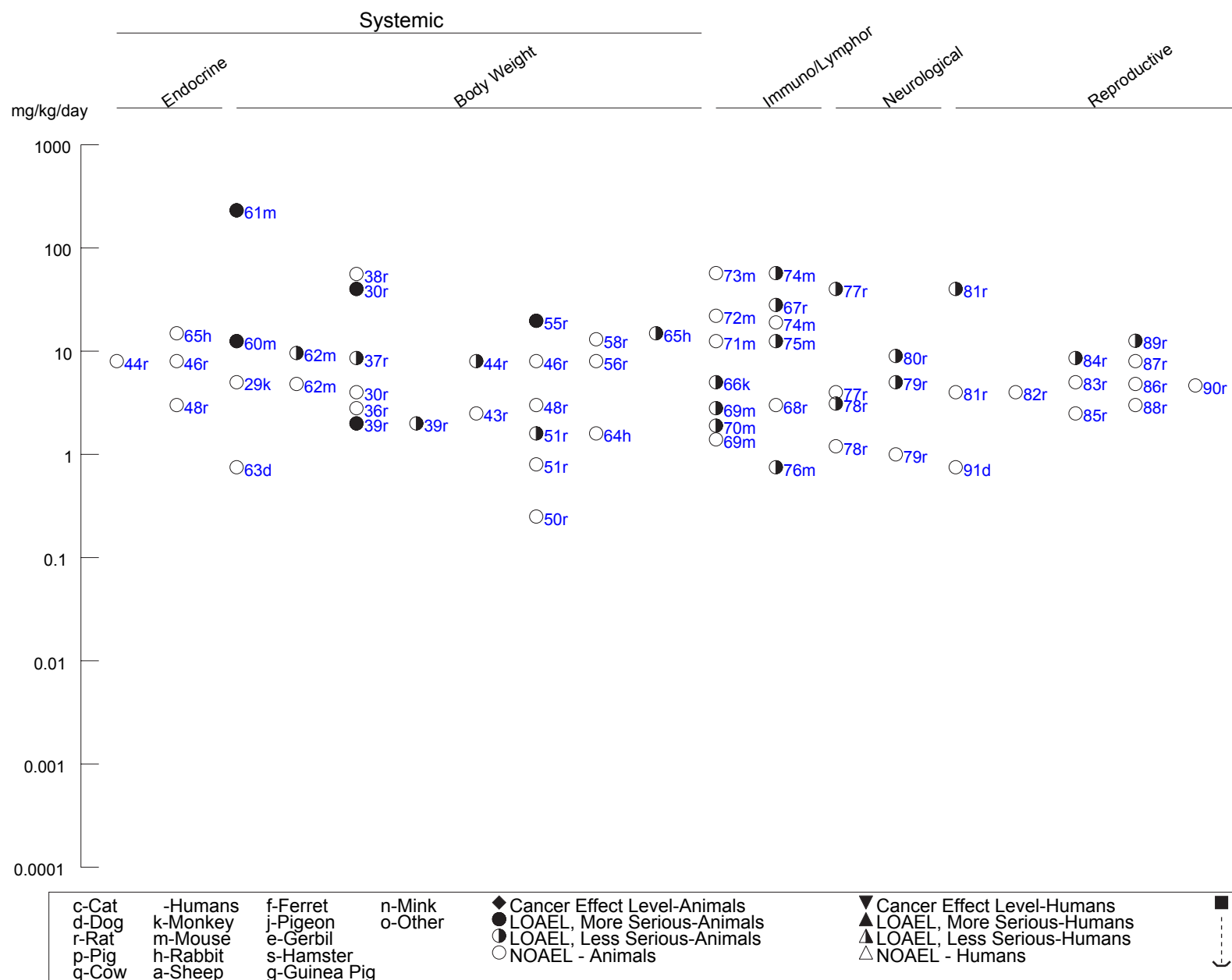
Figure 3-2 Levels of Significant Exposure to Cadmium - Oral (Continued) Intermediate (15-364 days)
