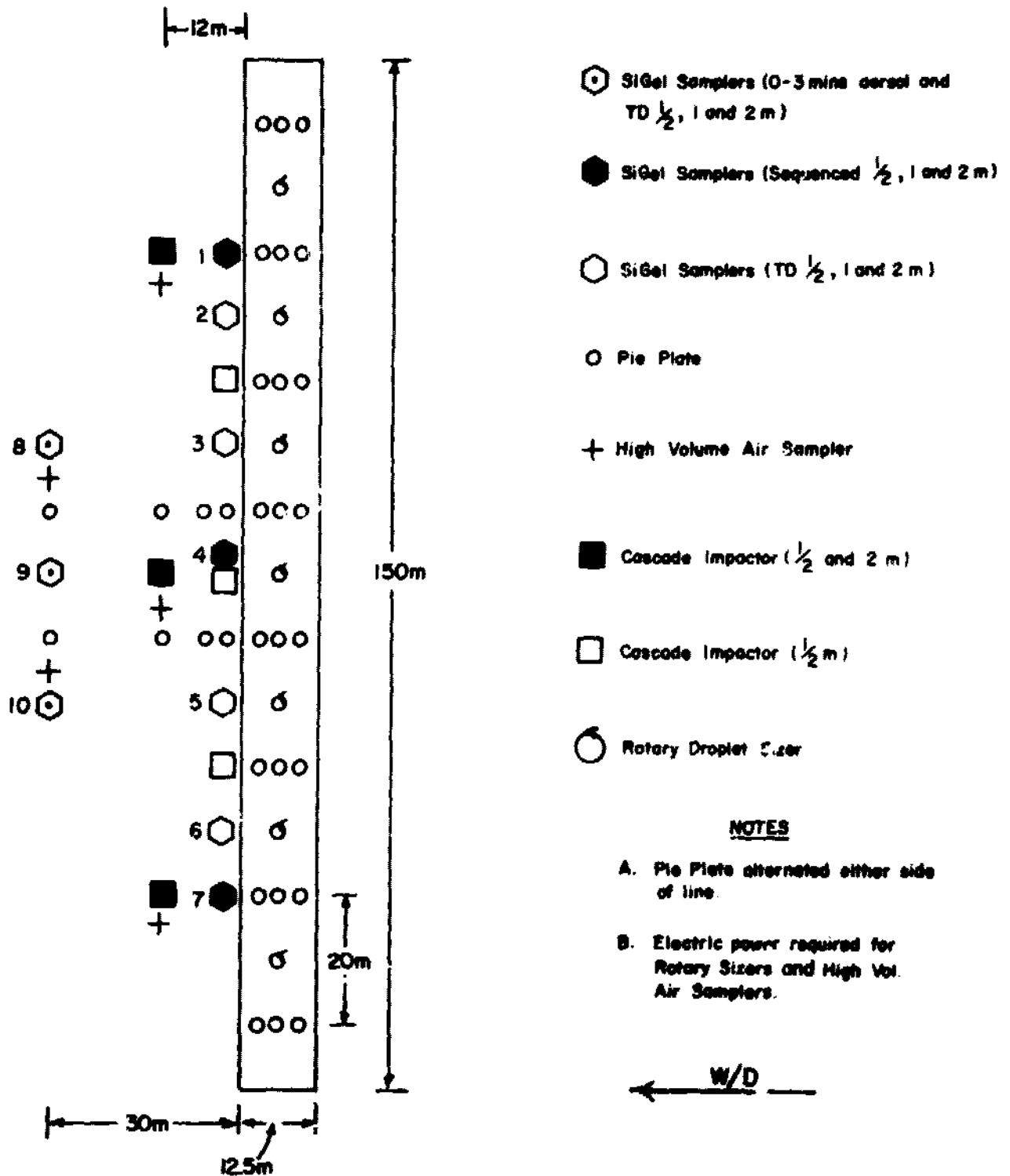
LAYOUT DIAGRAM F.E. 593 (TRIALS 15-22)
