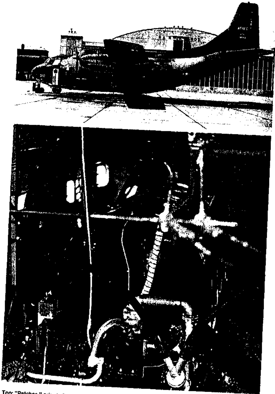
Top: "Patches," prior to its retirement, 1979; bottom: an A/A45Y-1 internal spray system mounted in a UC-123K.
