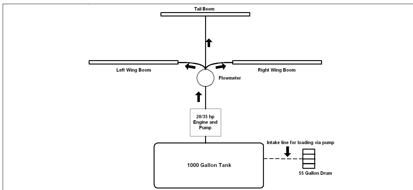
Fig. 1: A schematic of the C-123 'Provider' aircraft with internal spray system
