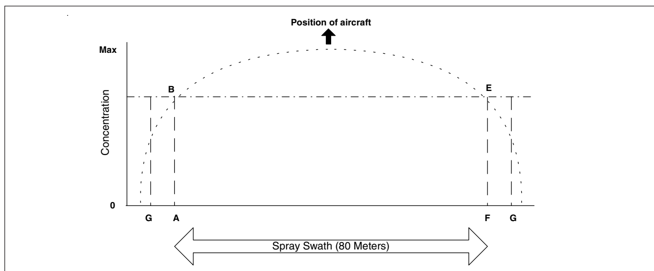
Fig. 2: A schematic cross-section of a deposition concentration profile perpendicular to the direction of flight. The spray system was the A/A45 Y-1 Internal Defoliant Dispenser interfaced with the UC 123 aircraft [adapted from Flynn, 5]. Dashed horizontal line is biologically effective concentration; dotted line is applied concentration
