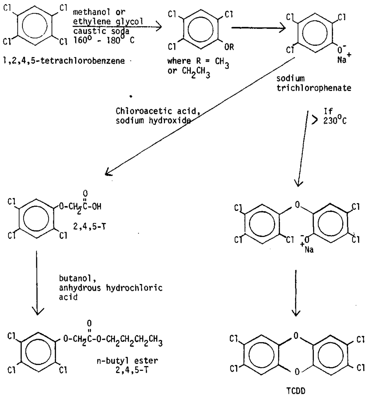
FIGURE 1. Synthesis scheme for production of the n-butyl ester 2,4,5-T (NBE 2,4,5-T) and site where formation of TCDD may occur.
