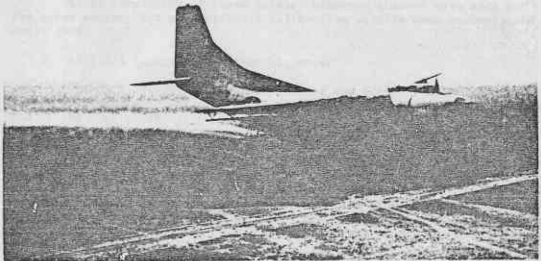
FIGURE 2. UC-123B Aircraft with MC-1 Spray System as Modified in the 1963 Egin AFB Calibration Trials.
