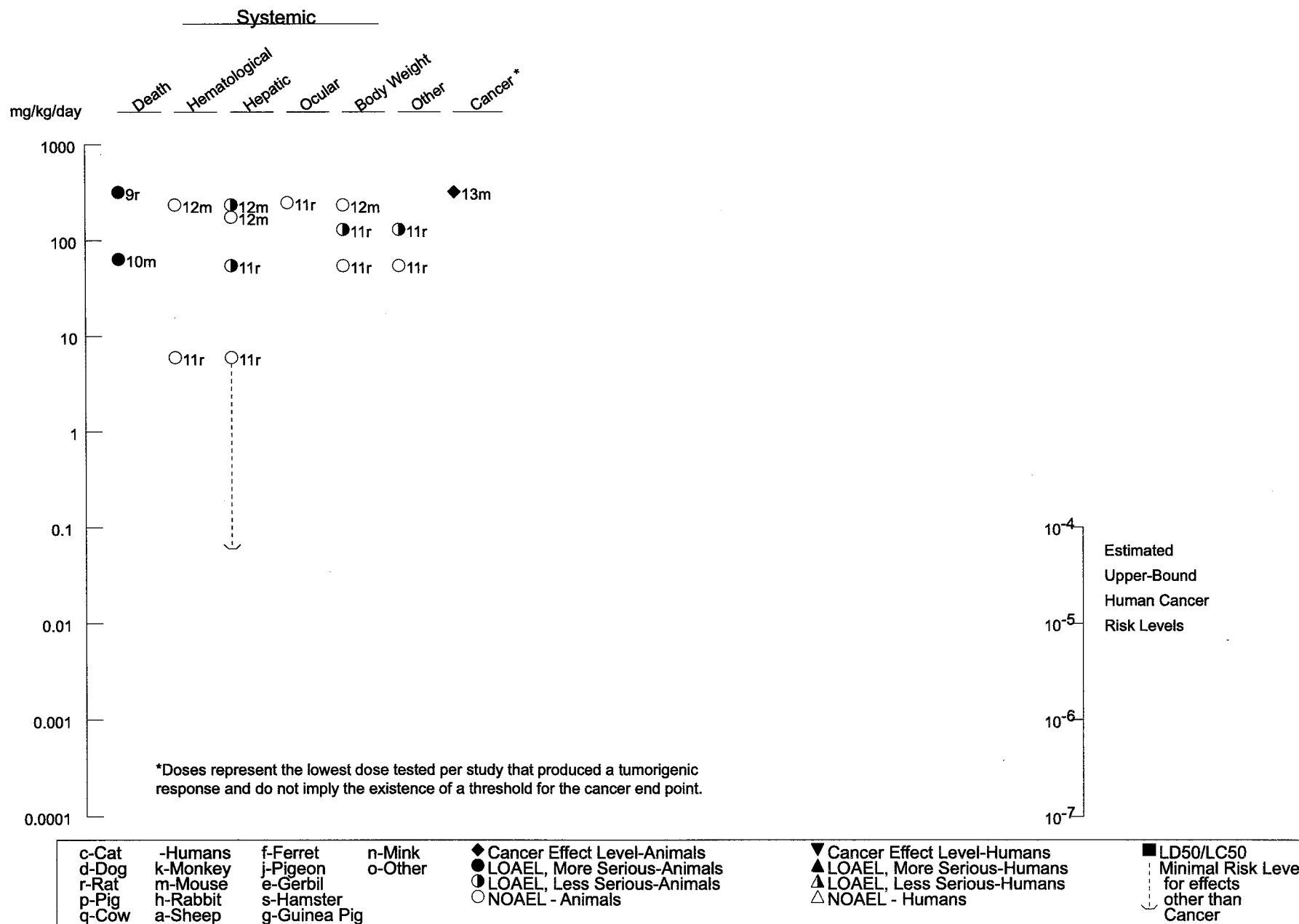
Figure 2-2. Levels of Significant Exposure to Methylene Chloride - Oral (continued) Chronic (≥365 days)
