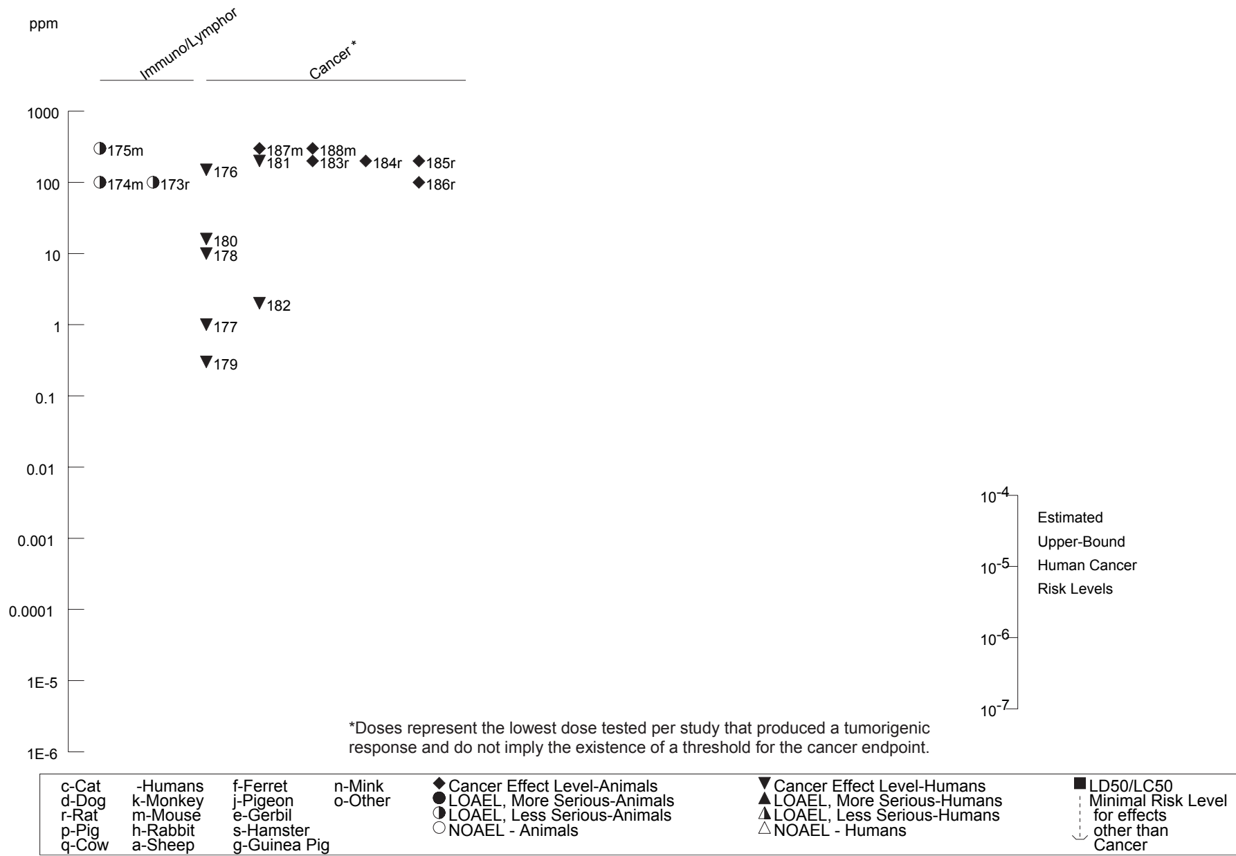
Figure 3-1 Levels of Significant Exposure to Benzene - Inhalation (Continued) Chronic (≥365 days)
