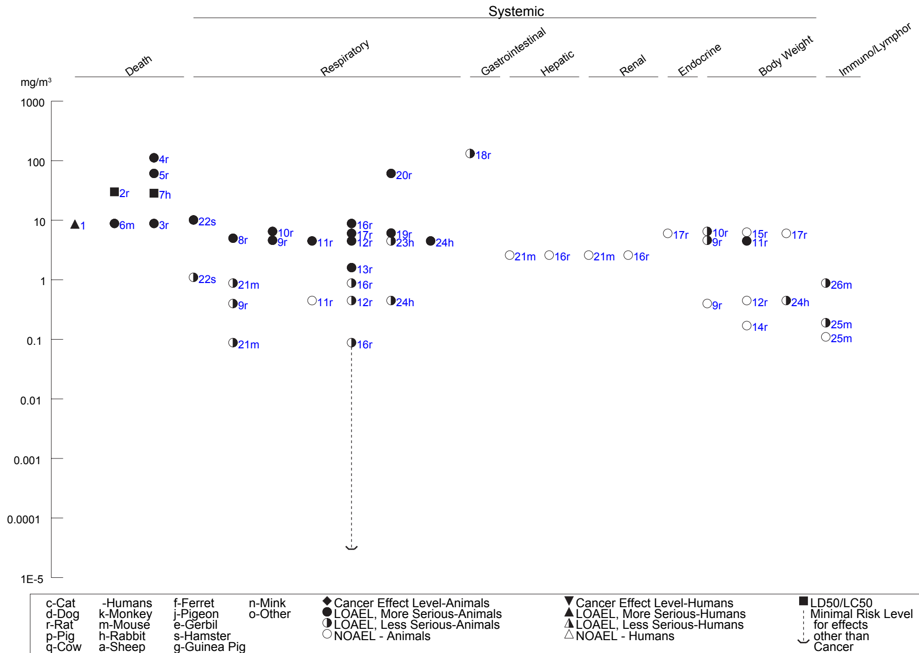
Figure 3-1 Levels of Significant Exposure to Cadmium - Inhalation
