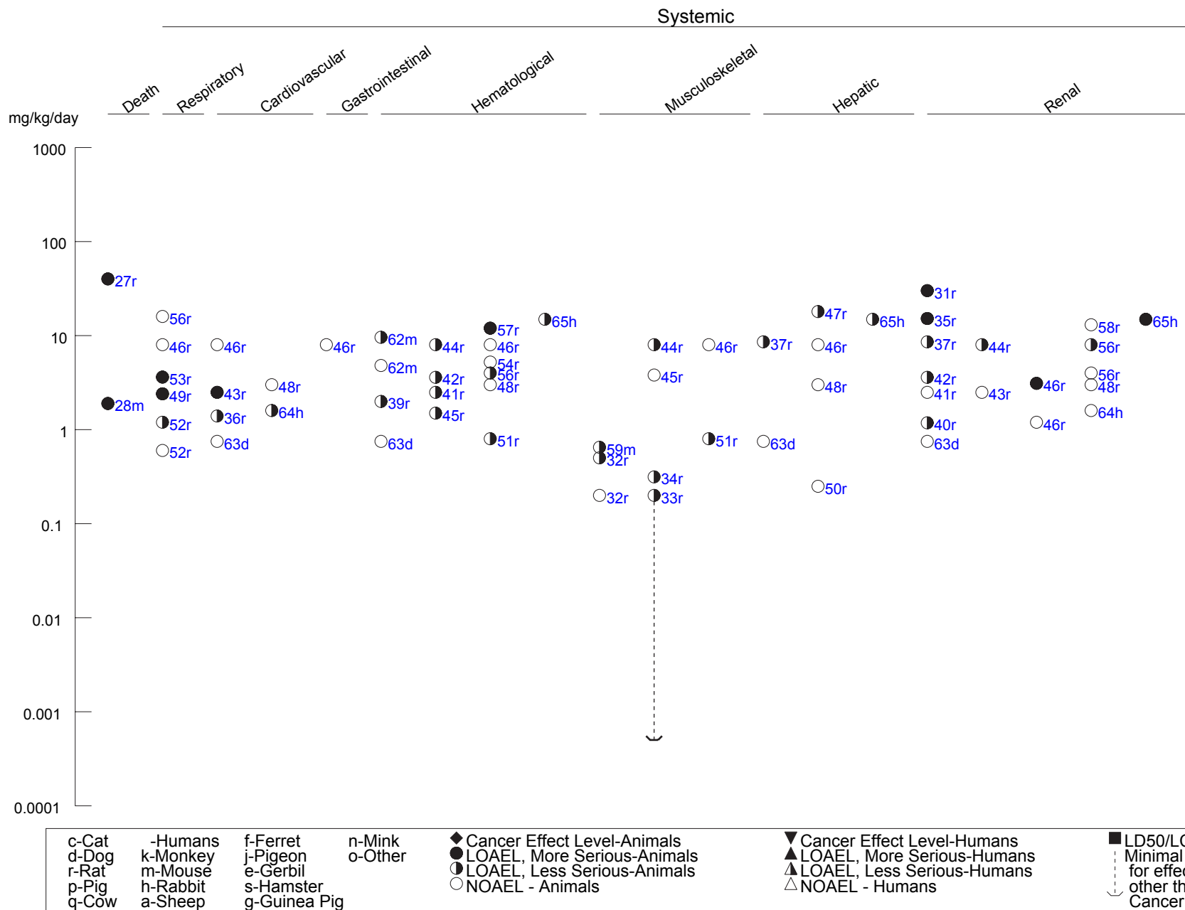
Figure 3-2 Levels of Significant Exposure to Cadmium - Oral (Continued)
