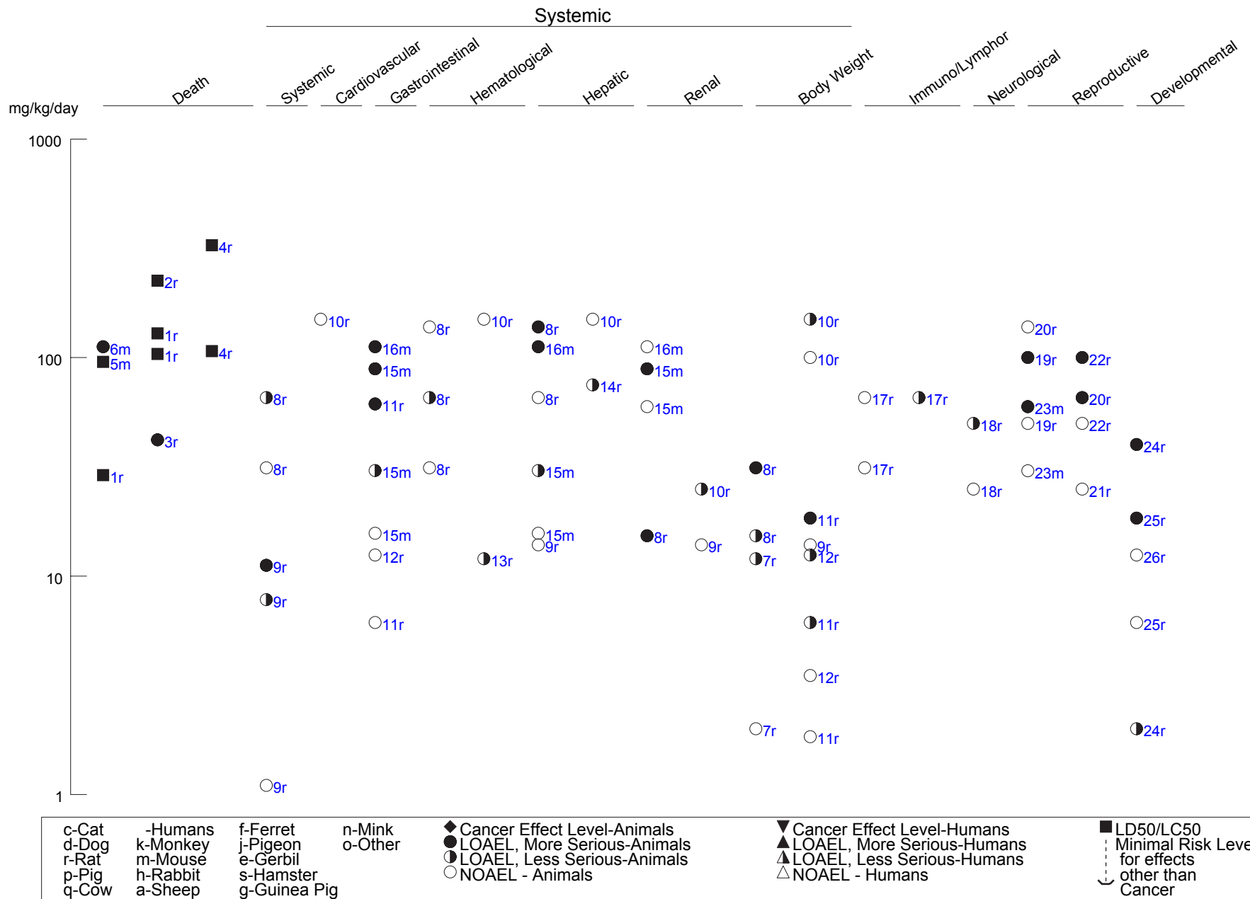
Figure 3-2 Levels of Significant Exposure to Cadmium - Oral
