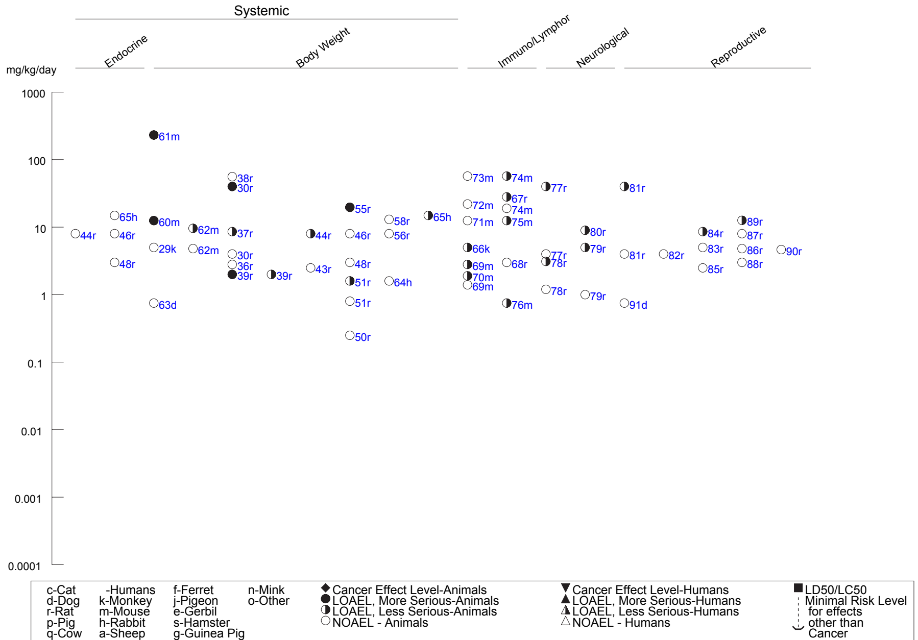
Figure 3-2 Levels of Significant Exposure to Cadmium - Oral (Continued) Intermediate (15-364 days)
