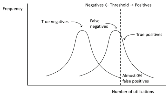
FIGURE 5-3 A classifier that minimizes the proportion of false positives.
