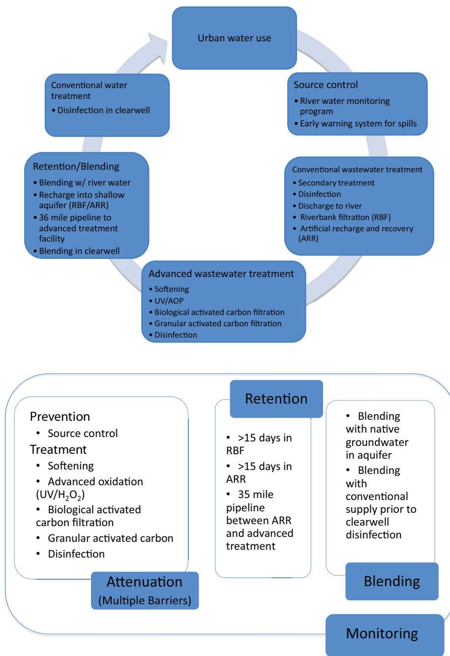
FIGURE 5-5 Case Study 3: Potable reuse design elements (including attenuation, retention, and blending) used for riverbank filtration of reclaimed water followed by softening, advanced oxidation, and carbon adsorption.
