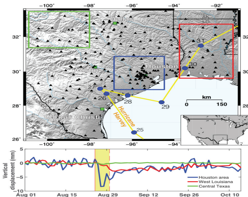
FIGURE 4.3 (Top) The path of Hurricane Harvey (yellow line) and its eye at noon (UTC), August 25–31, 2017 (blue dots), as it migrated across Texas and Louisiana. Black triangles are GPS stations. (Bottom) GPS motions from time series in Houston (blue), western Louisiana (red), and central Texas (green). The yellow shaded region marks the hurricane landings, with the first landing causing 8 mm of subsidence in Houston, followed by a 5-week period of uplift, and the second landing in Louisiana having smaller loading effects. SOURCE: Reprinted with permission of AAAS from Milliner et al., 2018. © The Authors, some rights reserved; exclusive licensee American Association for the Advancement of Science. Distributed under a Creative Commons Attribution NonCommercial License 4.0 (CC BY-NC) http://creativecommons.org/licenses/by-nc/4.0 .
