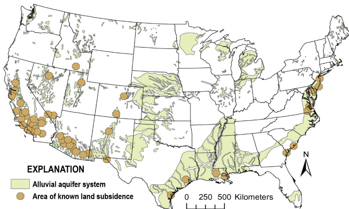
FIGURE 4.4 Areas where subsurface fluid withdrawal has caused land subsidence (brown) in the contiguous United States. SOURCES: Sneed, 2018, as modified from Clawges and Price, 1999, and Galloway et al., 1999.
