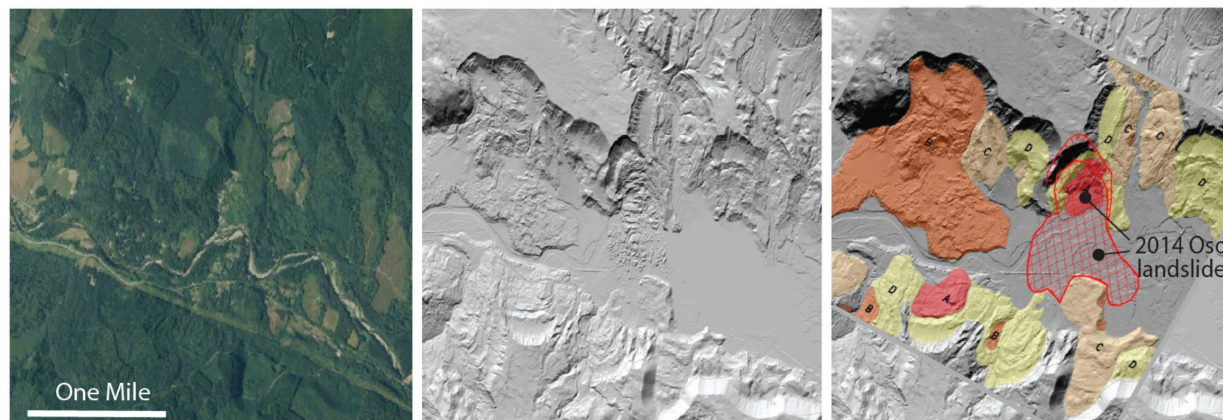
FIGURE 7.4 In the rain-soaked forests of Washington state (A), the density, extent, and frequency of destructive landslides were largely unrecognized until airborne lidar (B) was acquired after the 2014 Oso landslide, which killed 43 people. With vegetation removed, multiple generations of large landslides are obvious (C), and their relative ages are revealed both by cross-cutting relationships among them and by the relative roughness of their current topography. Older landslides become smoother over time. SOURCE: Haugerud, 2014.
