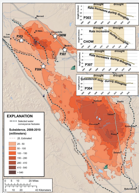
FIGURE 4.5 Spatial extent and magnitude of subsidence in the San Joaquin Valley for 2008–2010 as interpreted from InSAR data, and time series from four GNSS stations showing varying heights during drought and nondrought periods (inset). The complimentary data sets are needed to track subsidence spatially and temporally. SOURCE: Modified from Sneed et al., 2018.
