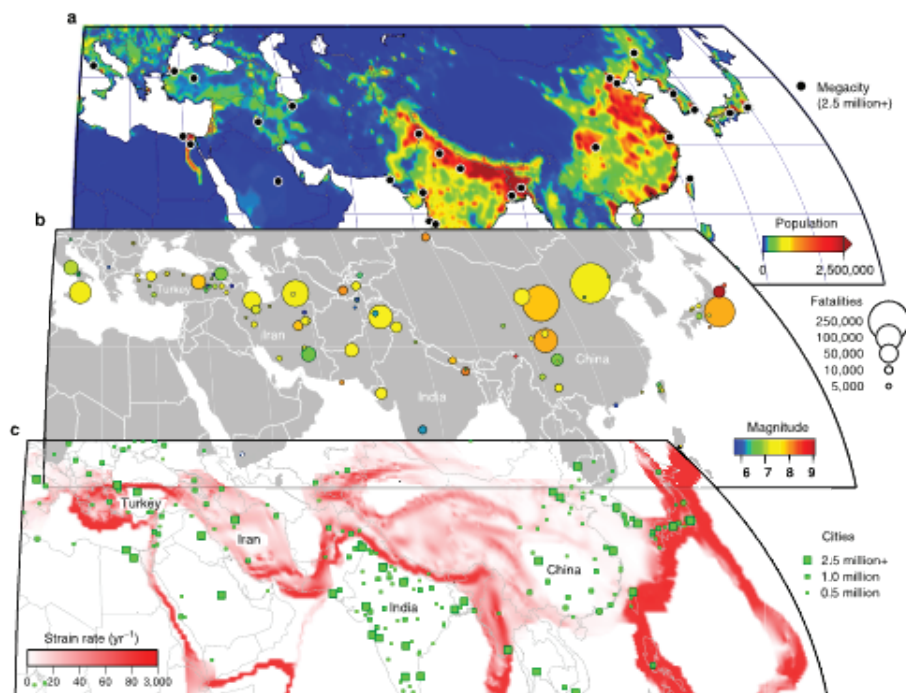
FIGURE 5.2 Population density, destructive earthquakes (> 1,000 fatalities), and crustal strain rate for Eurasia. Most large continental earthquakes occur in areas where the strain rate exceeds 50 nanostrain per year. Many of these areas are heavily populated and have had major destructive earthquakes in the past. The deformation of this large area is best monitored by a combination of Global Navigation Satellite System (GNSS) and Interferometric Synthetic Aperture Radar (InSAR). High-resolution topography would also reveal the paleoseismic activity on the many faults in the region. SOURCE: Elliott et al., 2016.
