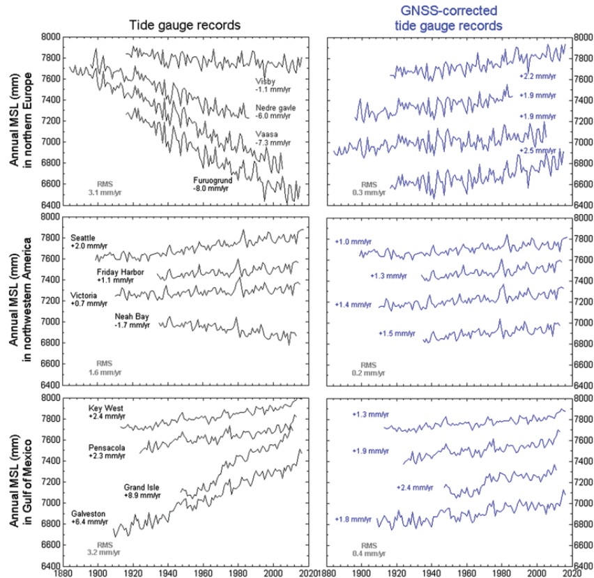
FIGURE 3.4 Relative sea-level rise at different sites measured by tide gauges. Left panels: uncorrected records. Right panels: records corrected for vertical land motions. SOURCE: Woodworth et al., 2019.
