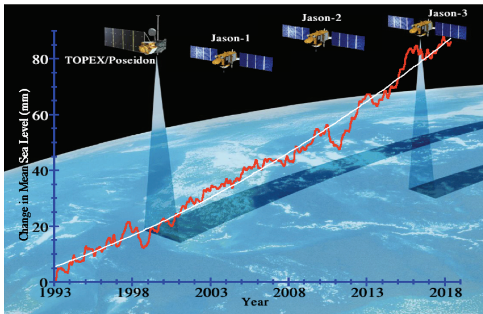
FIGURE 3.1 Altimetry record of global mean sea level from 1993 to present. The mean rate of rise is 3.1 \pm 0.3 mm/yr. The climate-driven acceleration, estimated after correcting for short-term natural variability (effects of volcanic eruptions and the El Niño–Southern Oscillation), is 0.084 \pm 0.025 mm/yr 2 . SOURCES: Modified from Beckley et al., 2017, and Nerem et al., 2018.
