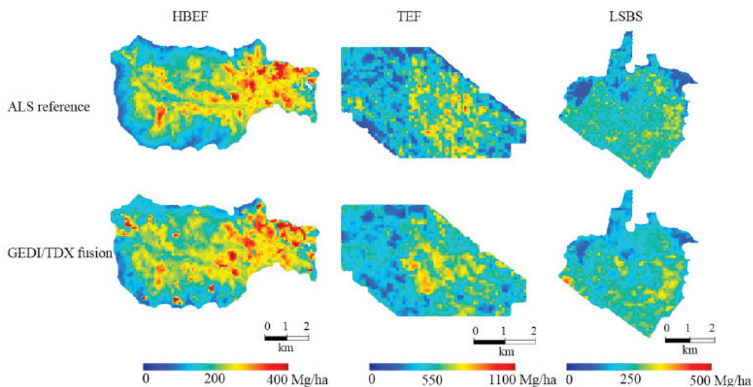
FIGURE 7.3 Airborne LiDAR System (ALS) is used as a reference for biomass estimates from GEDI and InSAR data from TerraSAR-X (2007) and TanDEM-X (2010) (abbreviated as TDX). Simulated GEDI and TDX data were fused to estimate biomass at 1 km scales, with uncertainties ranging from 7 percent to 12 percent. The three areas shown above are the Hubbard Brook Experimental Forest (HBEF, New Hampshire), Teakettle Experimental Forest (TEF, California), and the La Selva Biological Station (LSBS, Costa Rica). SOURCE: Reprinted from Qi et al., 2019, with permission from Elsevier.
