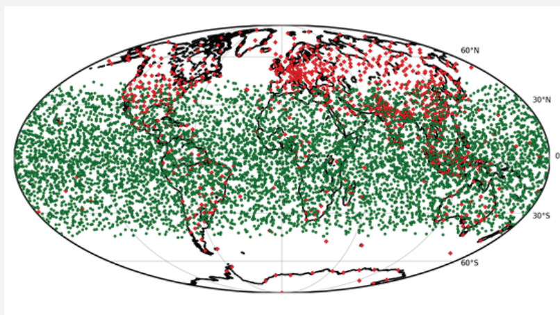
FIGURE 6.3 Locations of 4,000 occultations (green) for the COSMIC-2 constellation of 6 GNSS receivers orbiting at an altitude of 500 km and an inclination of 24^\circ . Ground-based radiosonde locations (red) only sample the atmosphere above land. SOURCE: https://www.cosmic.ucar.edu/what-we-do/cosmic-2 .
