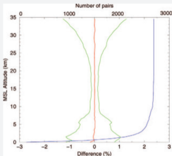
FIGURE 6.2 The precision of the index of refraction based on near-repeat occultations from two of the Constellation Observing System for Meteorology Ionosphere and Climate (COSMIC)-1 satellites. The red line shows the mean difference and the green lines show the standard deviation in percentage of difference. The number of paired occultations decreases at altitudes less than 5 km because of GNSS tracking errors, super refraction of the atmosphere, and low signal-to-noise of attenuation of the GNSS signal in the lower atmosphere. SOURCE: Anthes et al., 2008.
