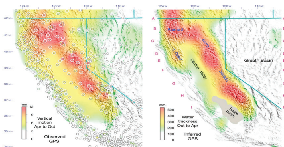
FIGURE 4.1 Vertical land displacement observed with the Global Positioning System (GPS) in the spring and summer (left) and the inferred change in total water storage, which increases in the fall and winter (right). Warm colors indicate higher amounts of uplift and greater amounts of water storage. Circles (left) indicate GPS sites. SOURCE: Argus et al., 2014.
