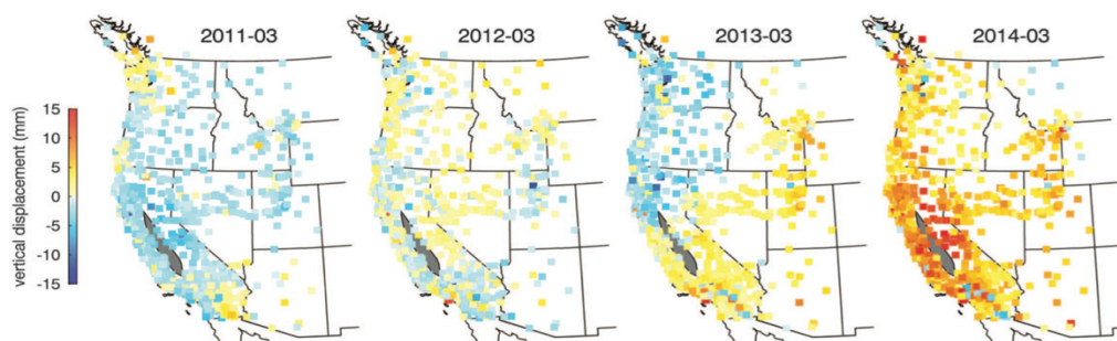
FIGURE 4.2 Vertical land displacements observed by GPS in the western United States from March 2011 through March 2014. The shift from land subsidence (blue) to land uplift (yellow and red) shows the effects of severe drought over the four-year period. Stations in the gray region (Central Valley of California) were excluded because groundwater-pumping induced land subsidence (see Box 4.2). SOURCE: Borsa et al., 2014.
